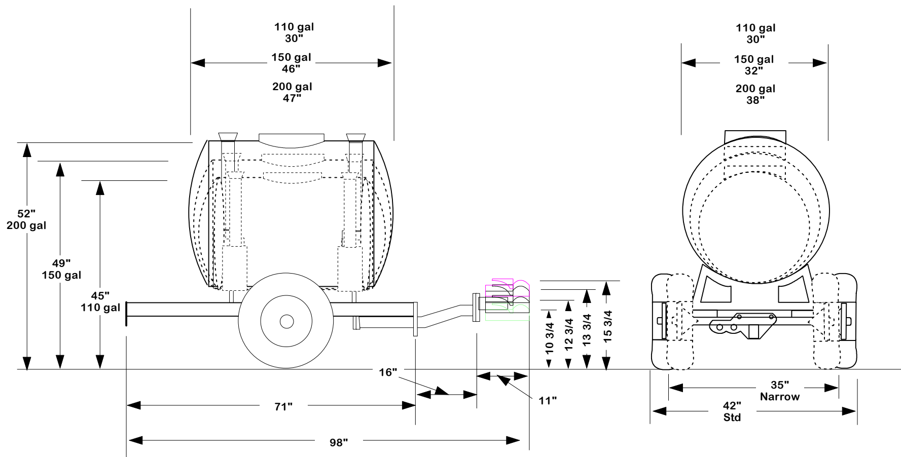
Trailer Dimensions Feed-R-Meter (9/19/2017)
